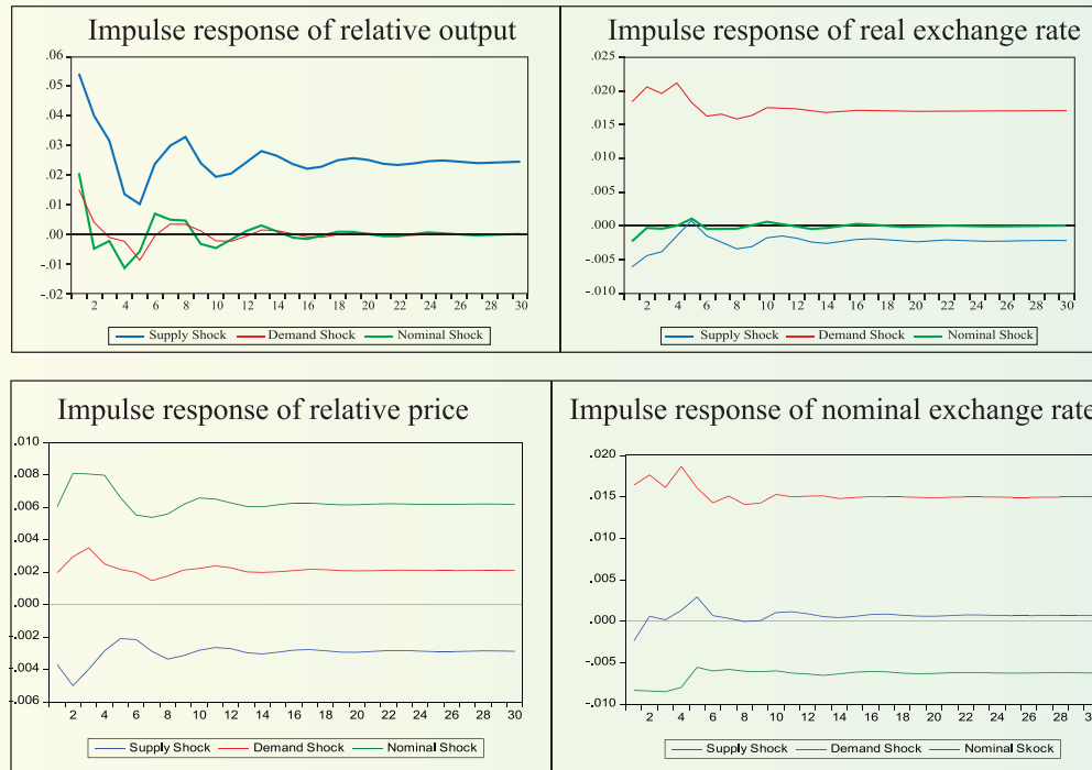
Fig. 15: Accumulated Impulse Response Function
