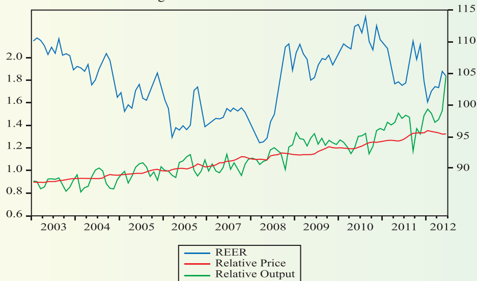
Fig. 14: Movements of variables
